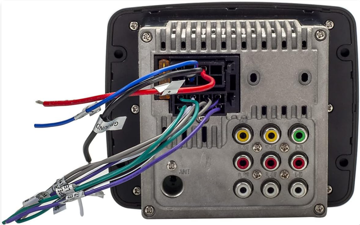
Figure 4.1: Rear panel connections of the RV3000.
