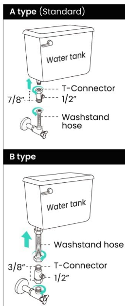
Image 4.2: A visual step-by-step guide for installation, covering removal of the old seat, base bracket installation, bidet seat placement, and water/power connections. It illustrates both Type A (standard) and Type B water tank connections.
