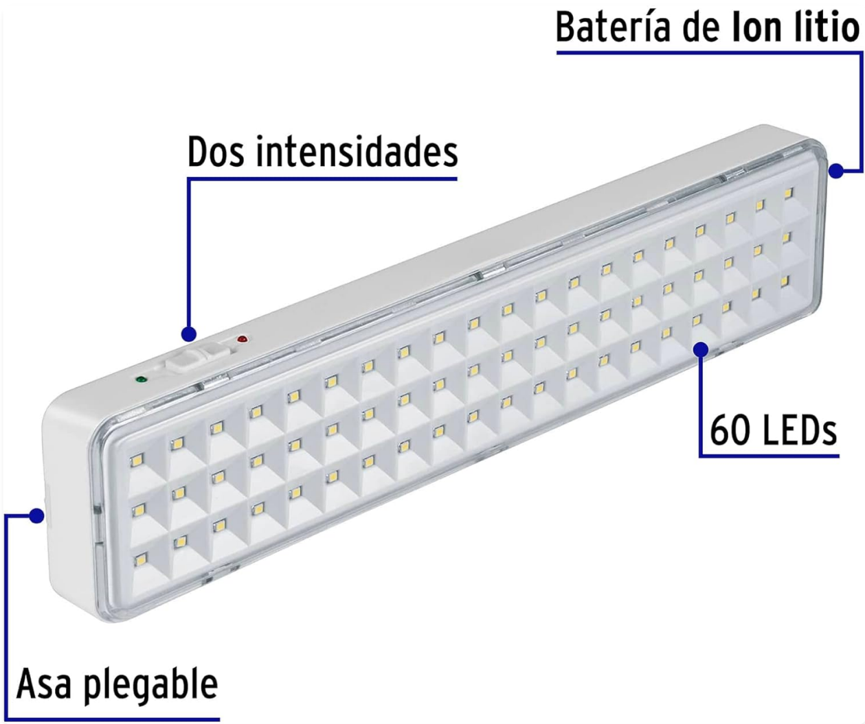
Figure 2: Key features of the Volteck LAE-60, including two light intensities, Lithium-Ion battery, 60 LEDs, and a foldable handle.
