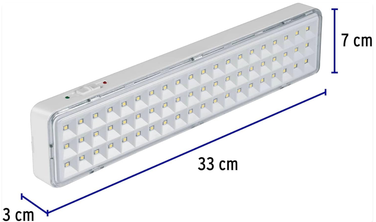
Figure 3: Dimensions of the Volteck LAE-60 emergency lamp: 33 cm length, 3 cm width, and 7 cm height.
