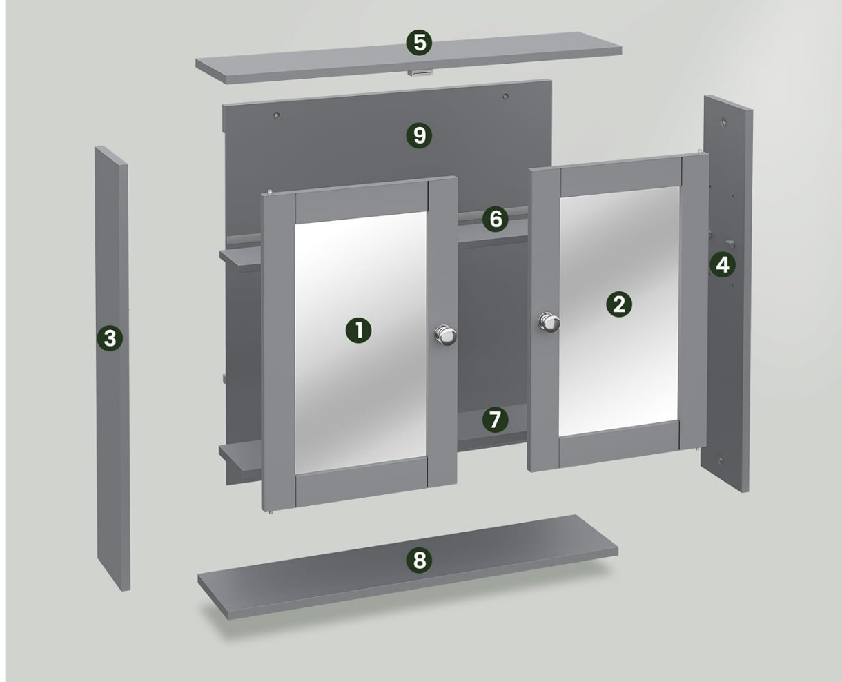
Image 3.1: Exploded view of the cabinet components with numbered labels for easy identification during assembly. The package typically includes:
