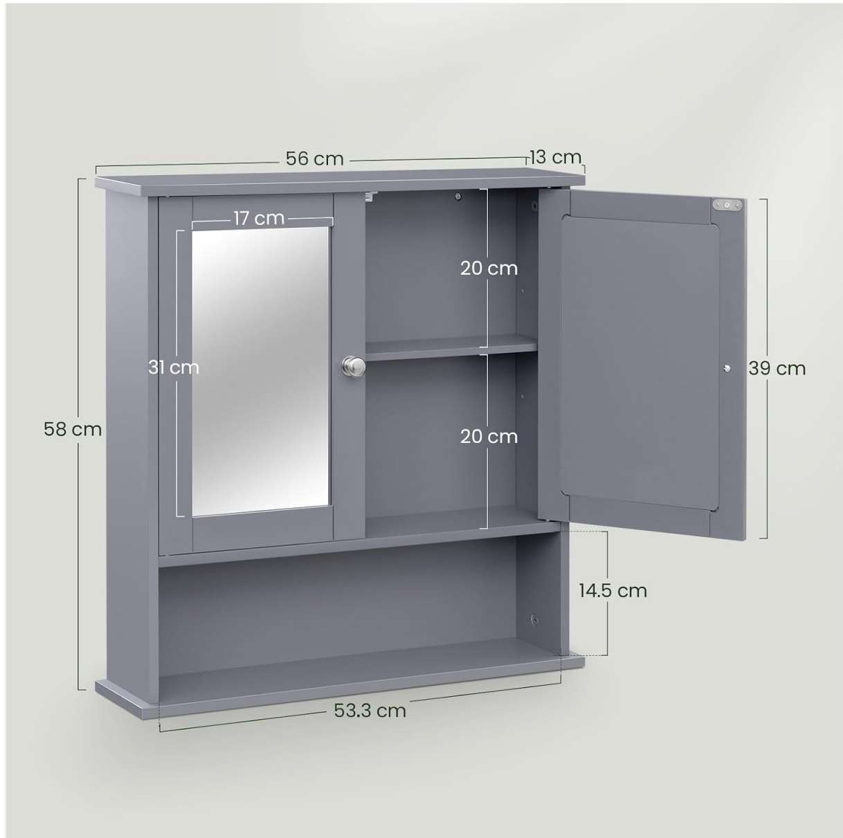
Image 4.1: Detailed dimensions of the cabinet, including overall size and mirror door measurements, useful for planning installation space.
