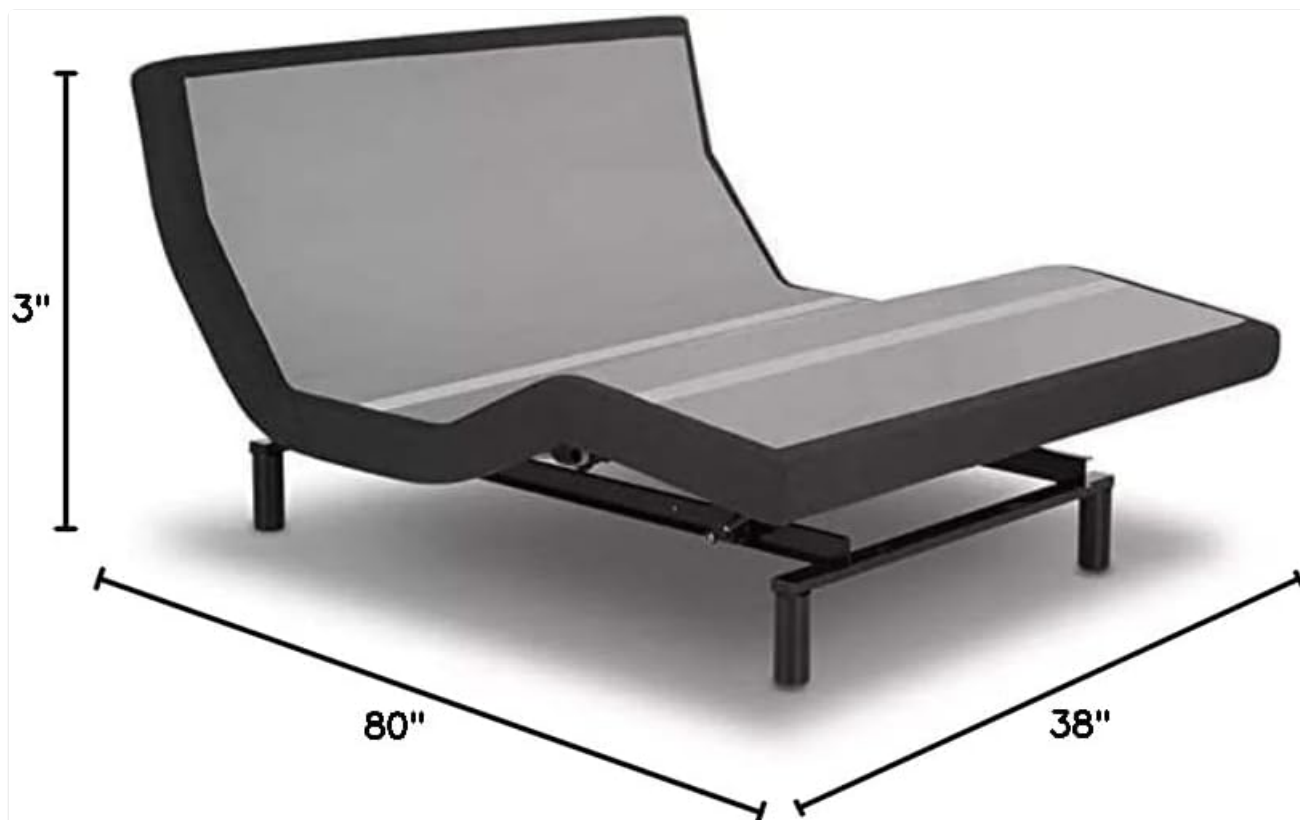
Figure 2: Dimensions of the Twin XL Prodigy PT Adjustable Base. The base measures approximately 80 inches in length, 38 inches in width, and 3 inches in height (excluding legs).
