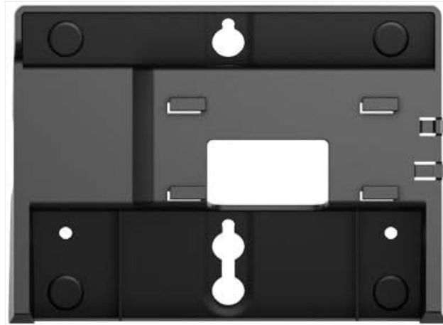
Figure 1: Rear view of the Fanvil WB101 Wallmount Bracket. This image displays the keyhole slots for wall mounting at the top and bottom, along with additional screw points and clips designed to secure a compatible Fanvil phone.
