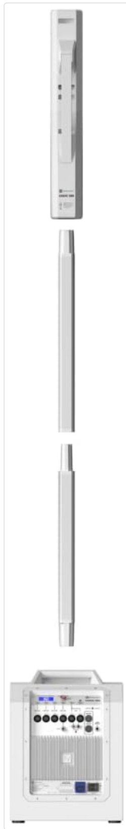
Figure 2.1: Exploded view showing the subwoofer, pole, and column array components.
