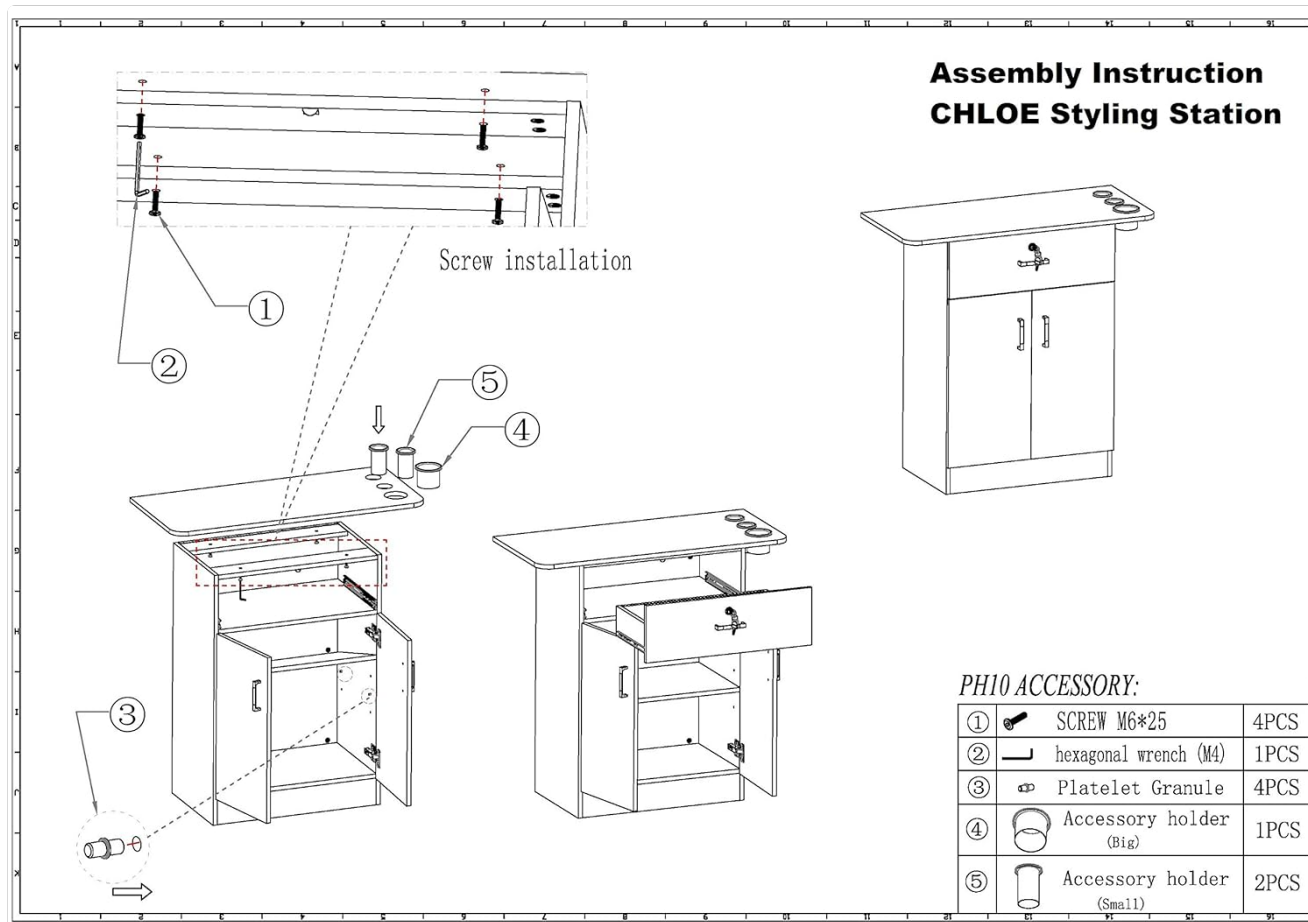
Image 3.1: Assembly instruction diagram for the CHLOE Styling Station. This diagram illustrates the various components and hardware required for assembly, including screws, a hexagonal wrench, platelet granules, and accessory holders.
