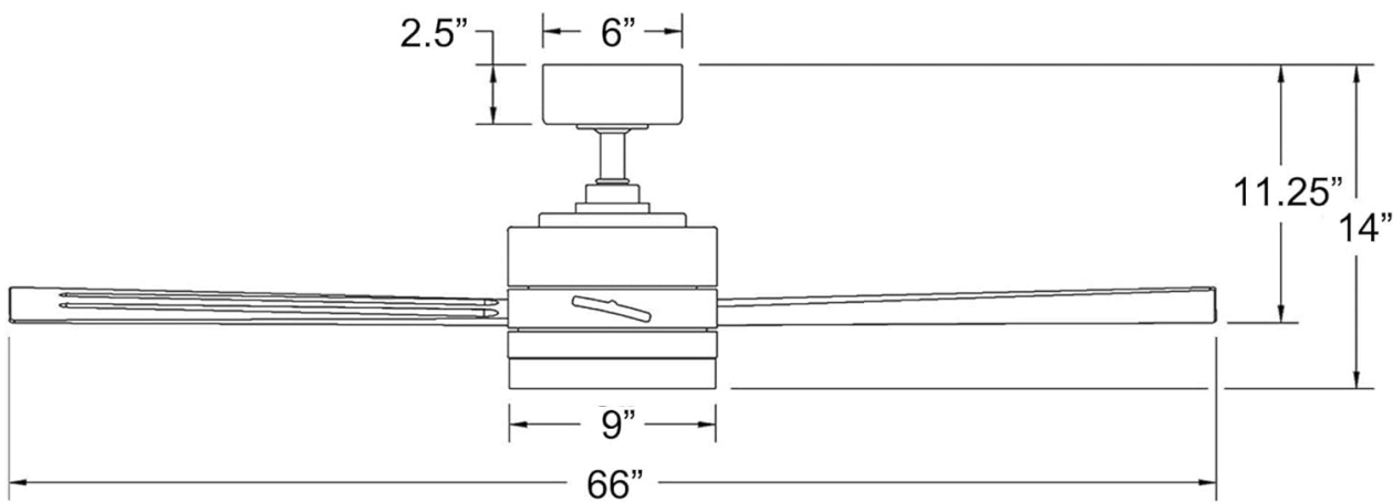
Figure 3: Fan Dimensions
