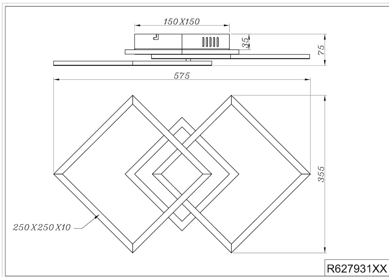
Figure 4.1: Technical drawing showing the dimensions of the R62793132 Venida LED Ceiling Light. Dimensions are approximately 57.5 cm (length) x 35.5 cm (width) x 7.5 cm (height).
