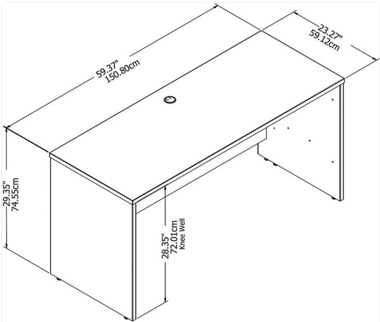
Image 2.1: Dimensional diagram of the Studio C Credenza Desk, illustrating overall size and knee well clearance.
