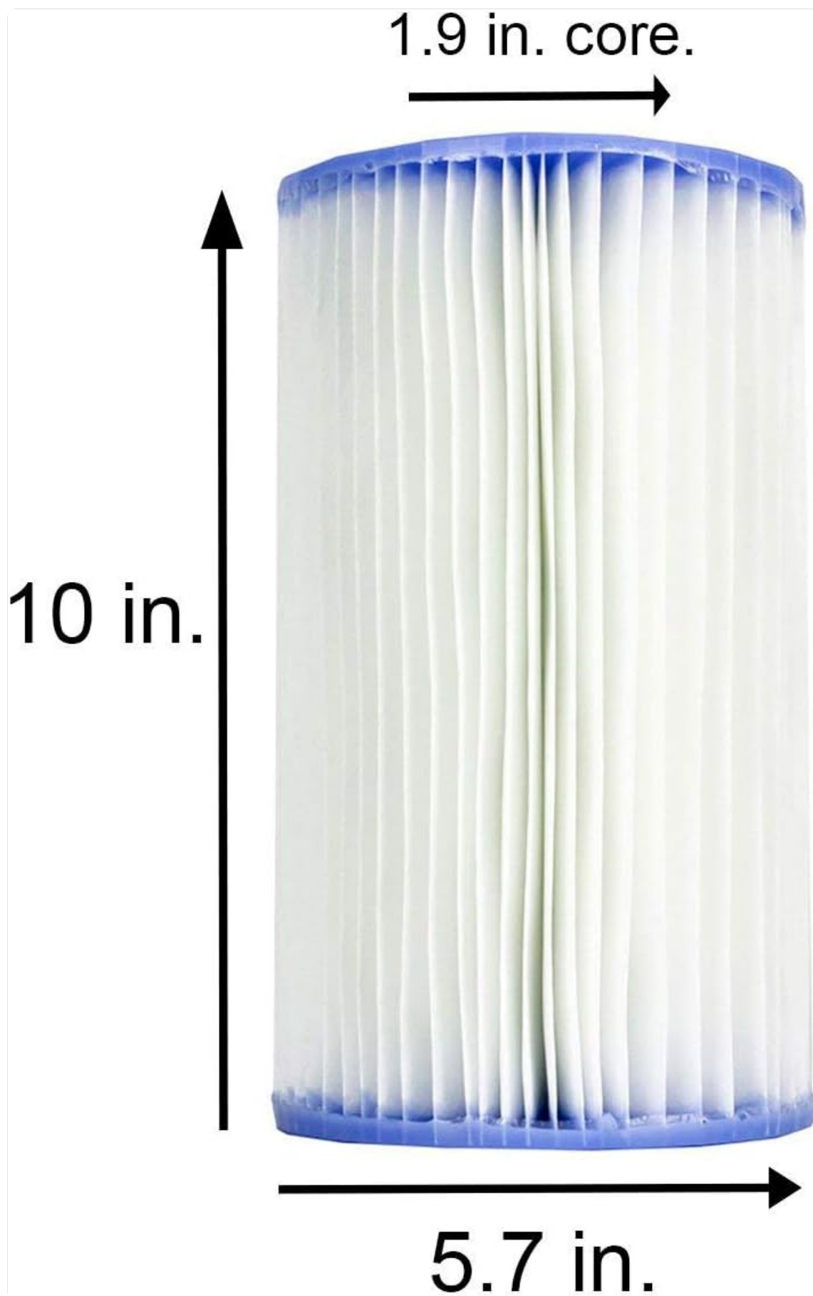
Image: Detailed dimensions of the Intex Type B filter cartridge.
