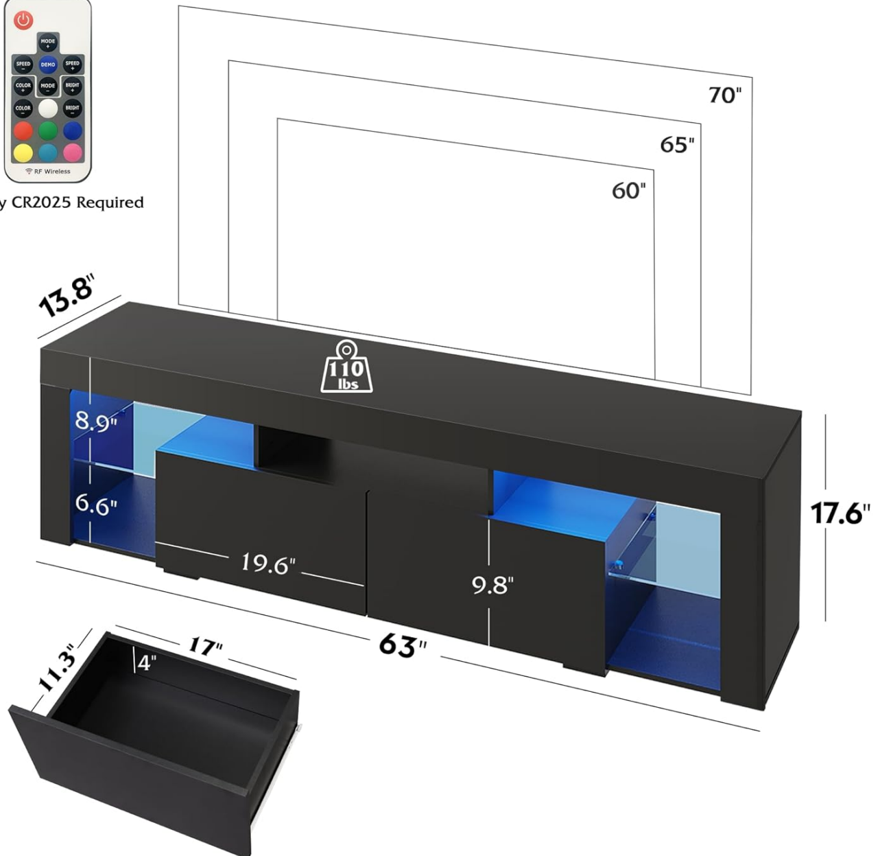
Image 7.1: Detailed product dimensions.
