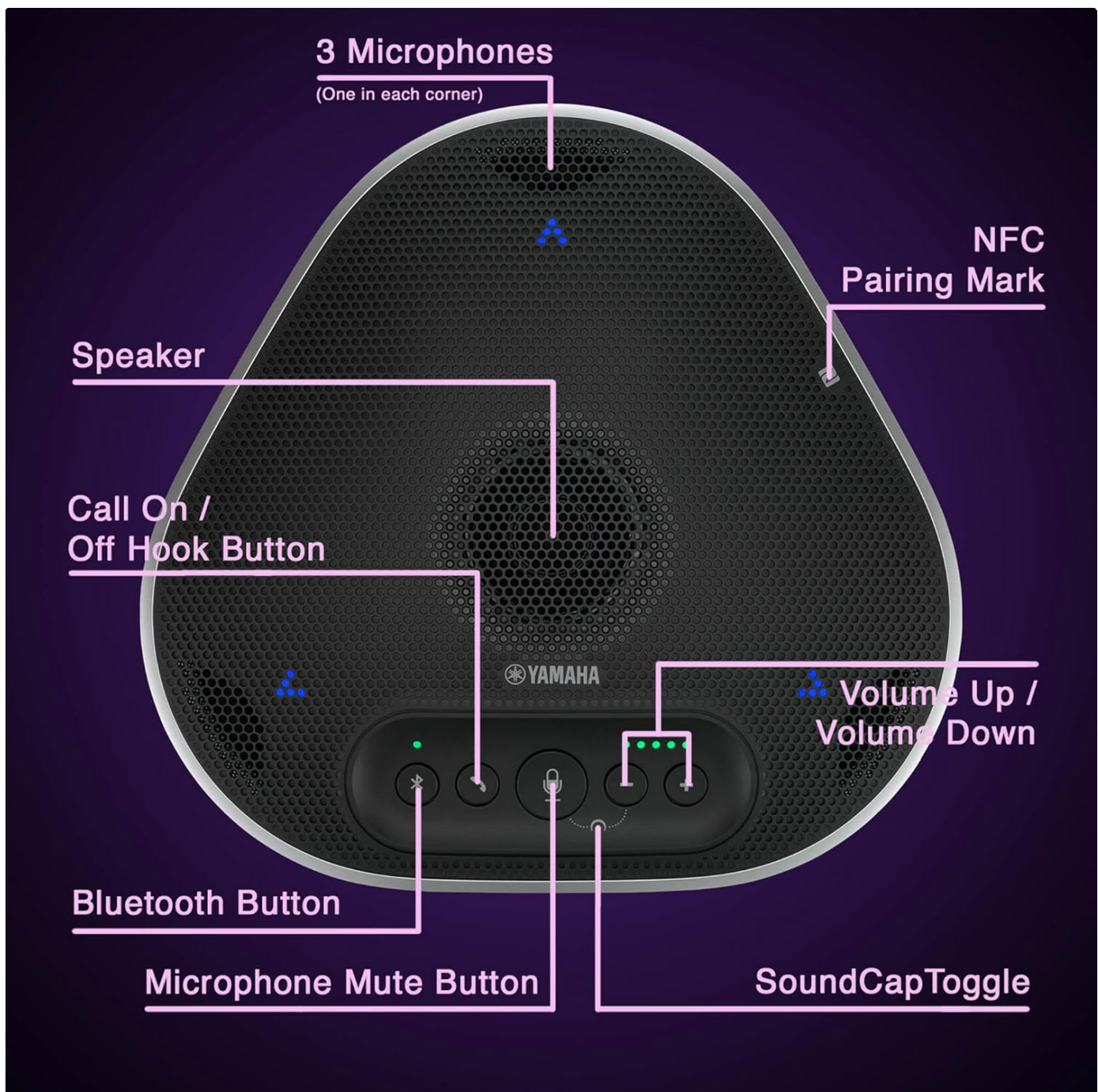
Image: A detailed diagram of the Yamaha YVC-330's top panel, with labels pointing to the 3 Microphones, NFC Pairing Mark, Speaker, Call On/Off Hook Button, Volume Up/Down, Bluetooth Button, Microphone Mute Button, and SoundCap Toggle.
