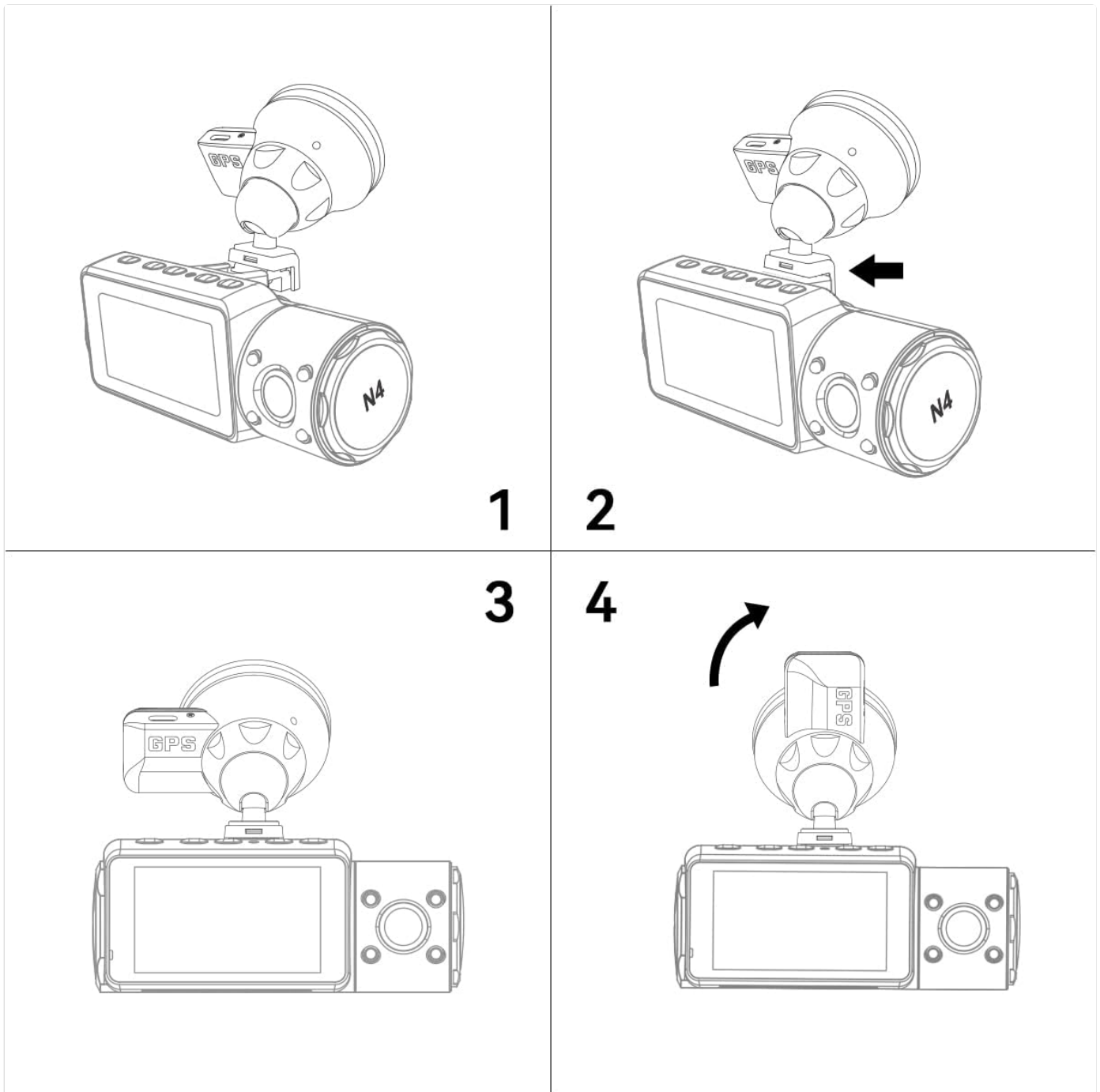
Figure 2: Step-by-step installation guide for the GPS module.
