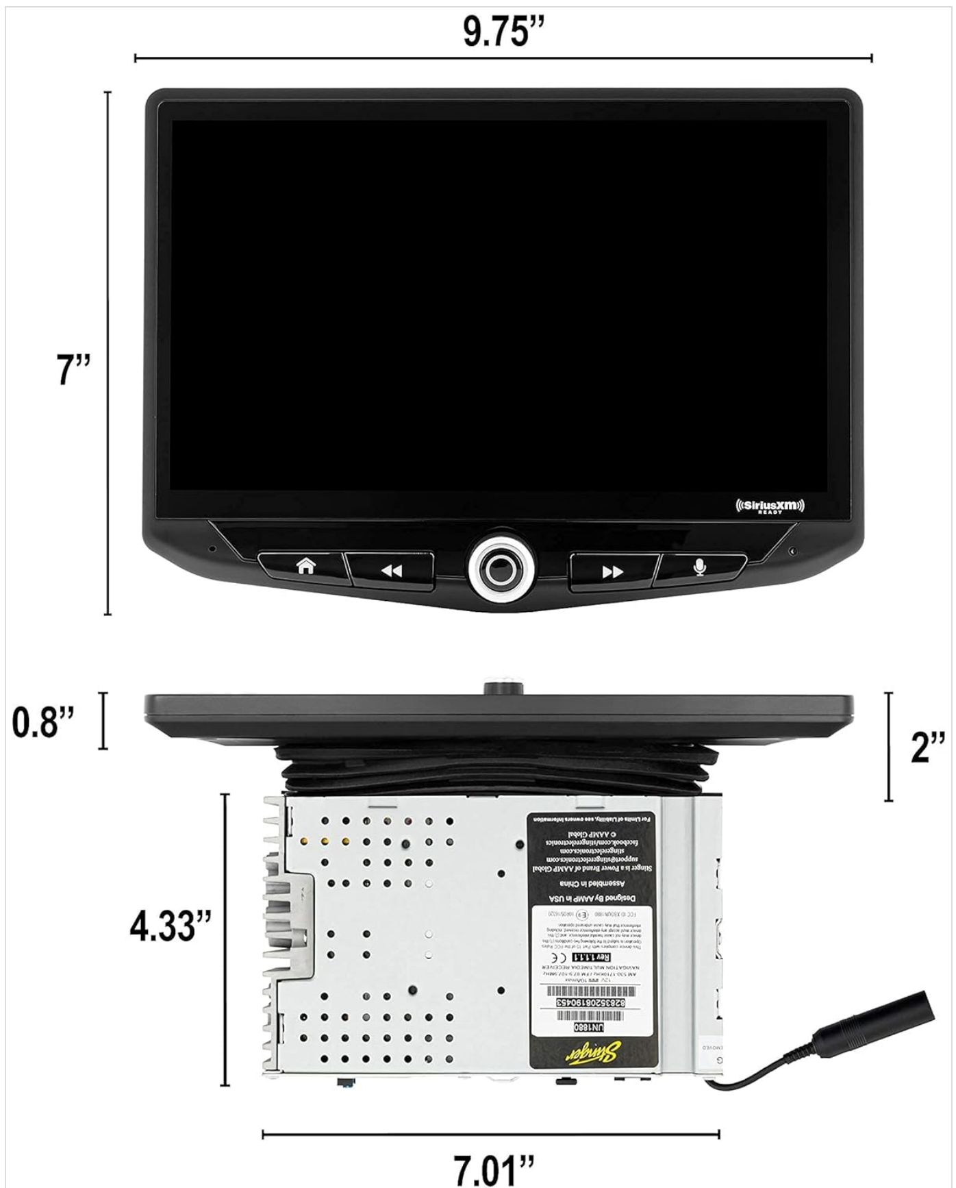
Image: A technical diagram illustrating the precise dimensions of the Stinger HEIGH10 unit, including its width, height, and depth, crucial for fitment and installation planning.
