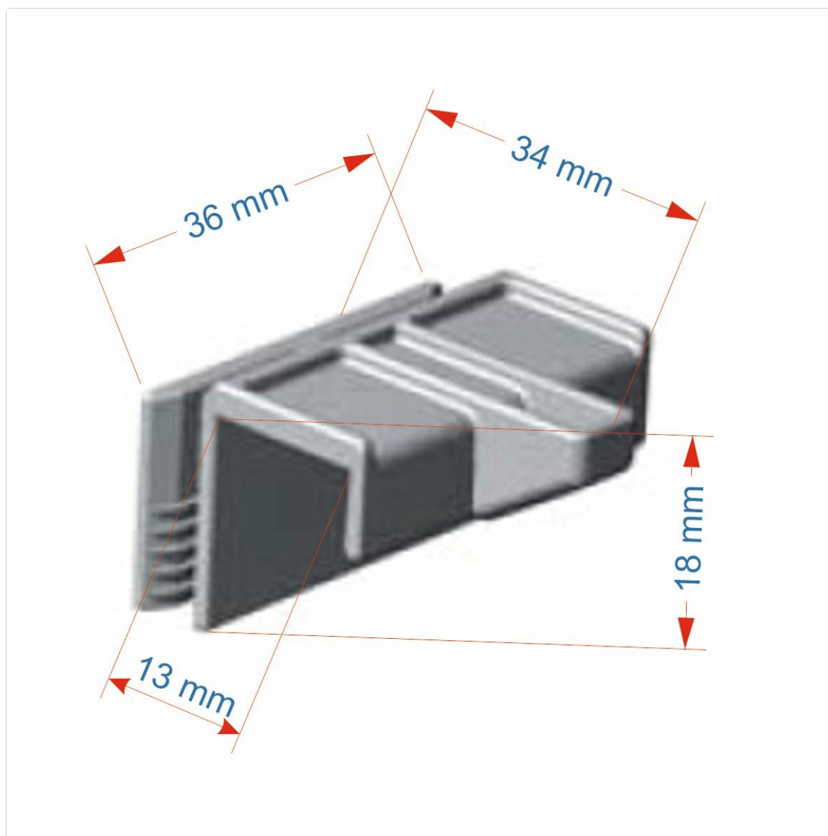
Image 3.1: Dimensional drawing of the plinth bracket.
