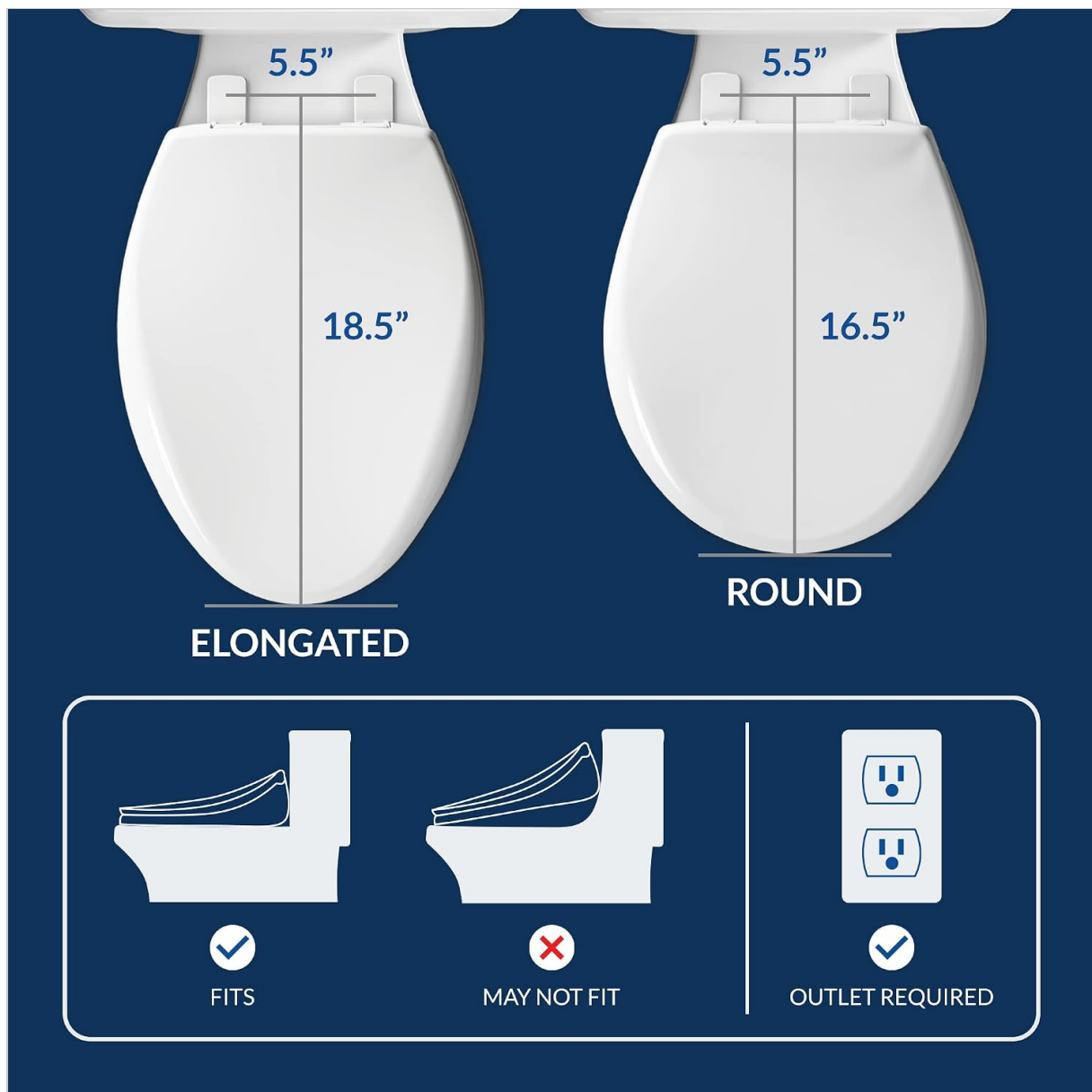
Image: Toilet seat dimensions for round and elongated models. The Bio Bidet U770 R is compatible with round toilets (16.5 inches from bolt to rim) and requires a nearby electrical outlet.
