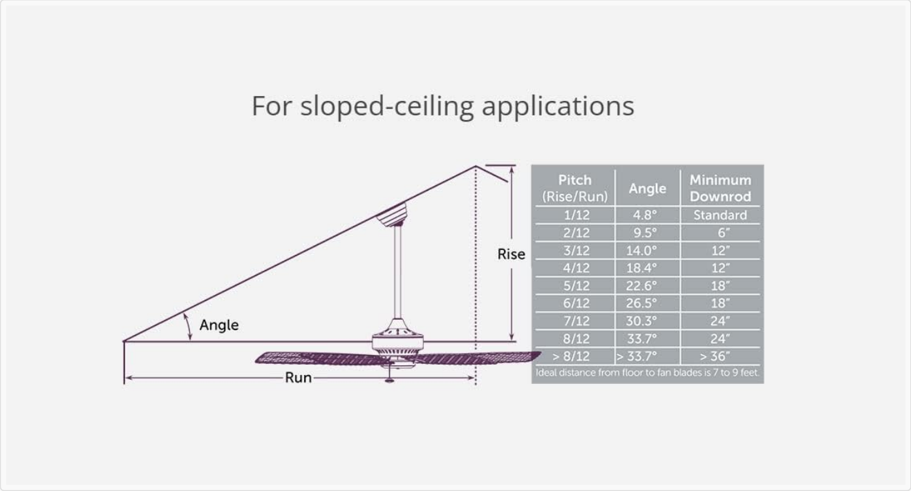
Image 2.1: Diagram illustrating a ceiling fan installation on a sloped ceiling, showing the pitch, angle, and recommended minimum downrod lengths for various ceiling slopes.
