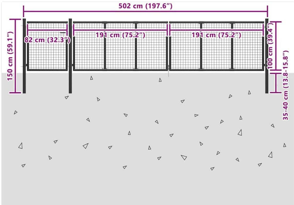
Image: Technical drawing showing the dimensions of the gate (502 cm width, 150 cm total height, 100 cm panel height) and recommended installation depth for posts.
