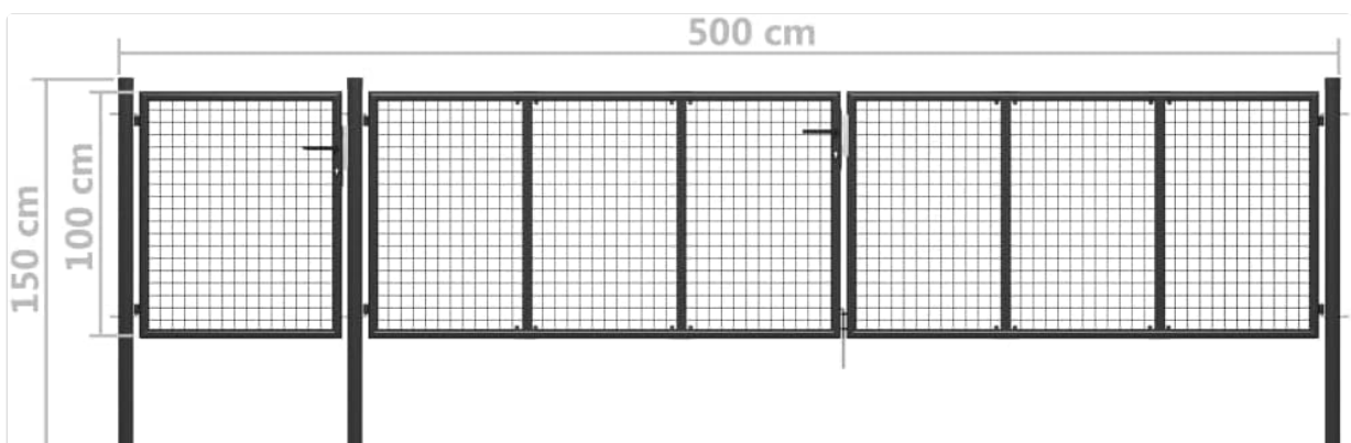
Image: An alternative view of the gate's dimensions, indicating overall width (500 cm) and total height (150 cm).
