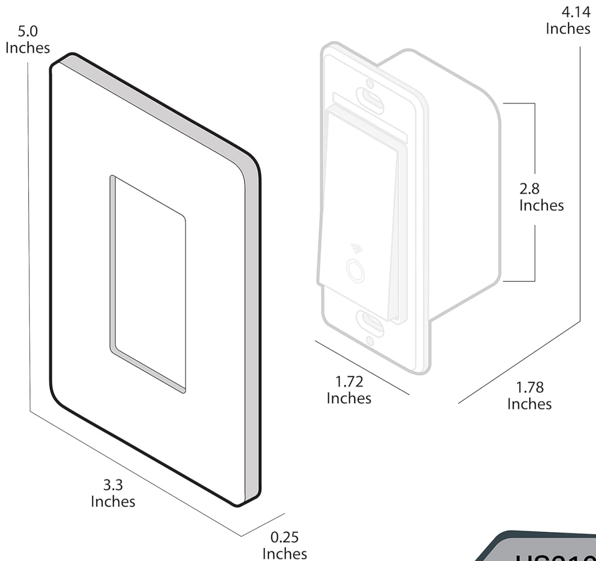
Image: Diagram illustrating the physical dimensions of the Kasa Smart HS210 switch.
