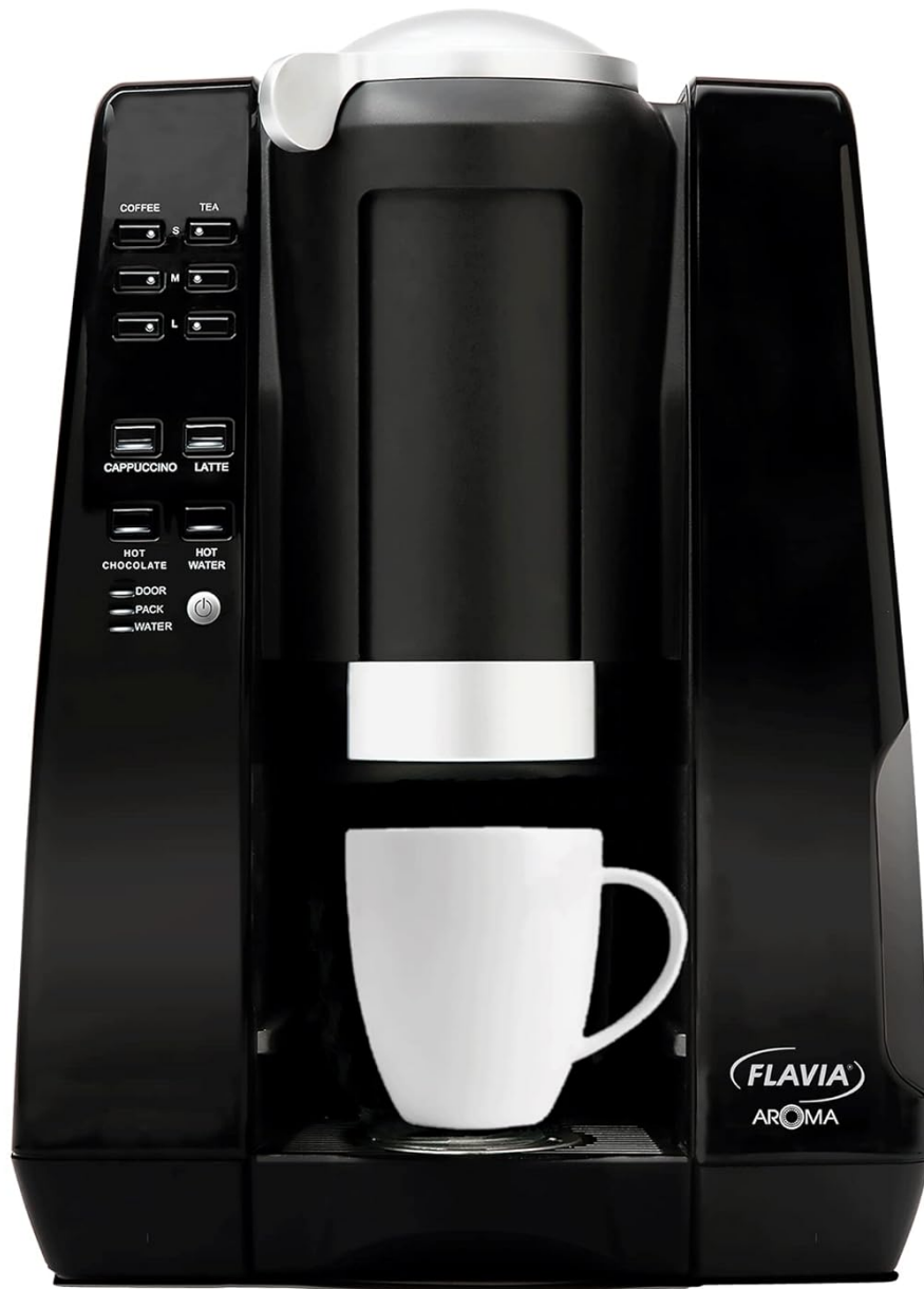
Image 3.1: Front view of the Flavia Aroma Single Serve Coffee Brewer. This image displays the main body of the brewer, including the control panel with various beverage selection buttons, the Freshpack insertion slot, the cup stand, and the drip tray.
