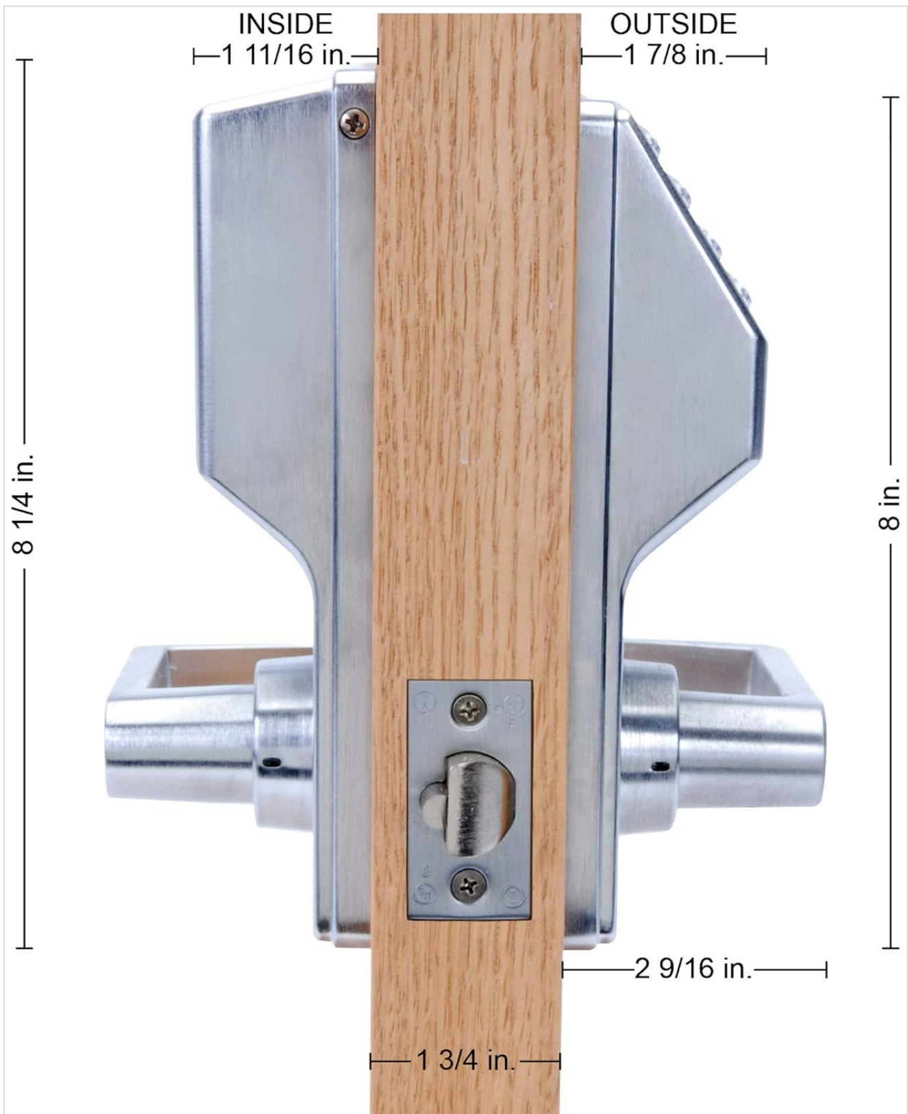
Figure 2: Installation dimensions for the Alarm Lock Trilogy T2 DL2700/26D.
