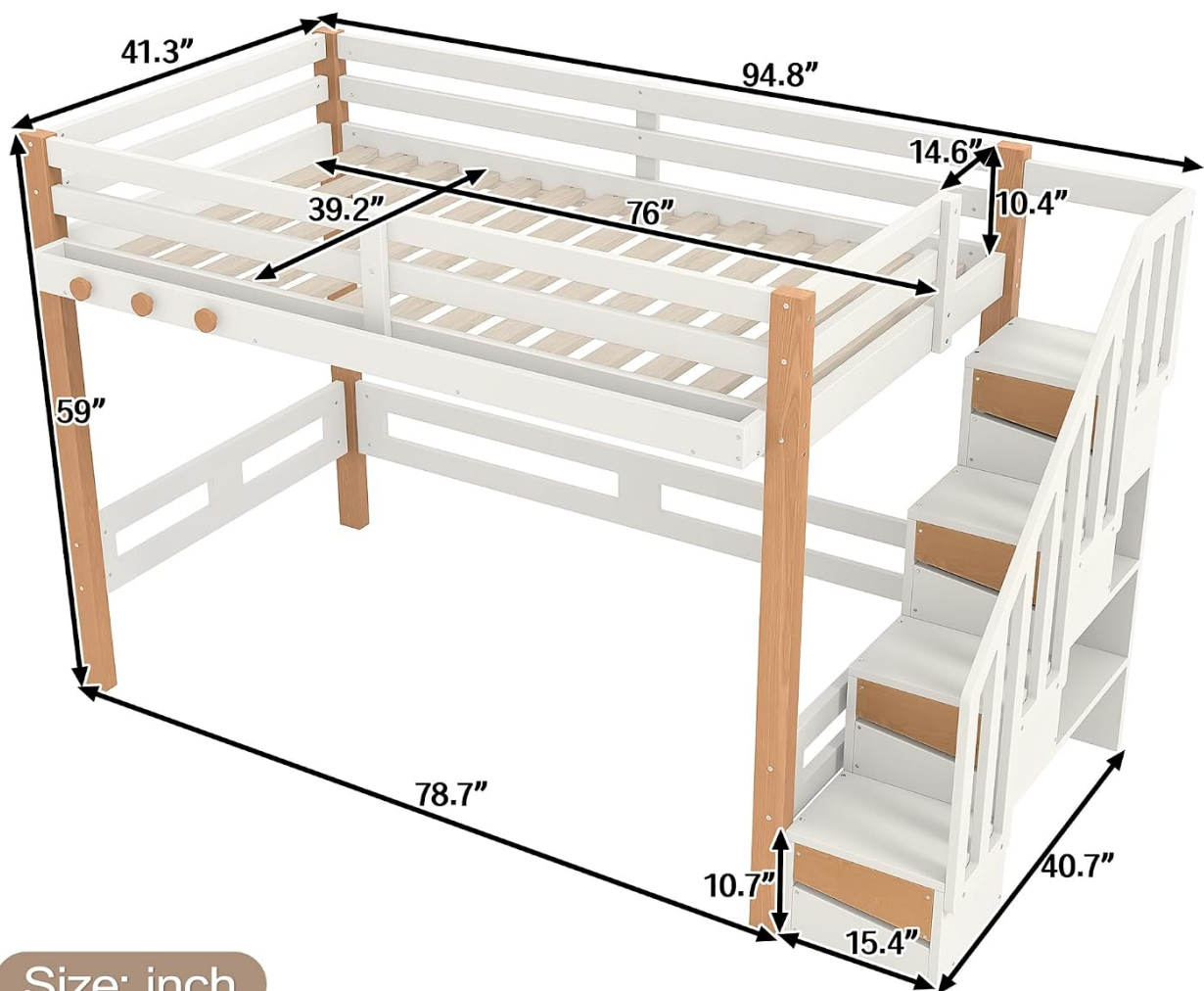
Image 3.1: Detailed product dimensions for the Bellemave Twin Loft Bed. Refer to this diagram during assembly and for space planning.
