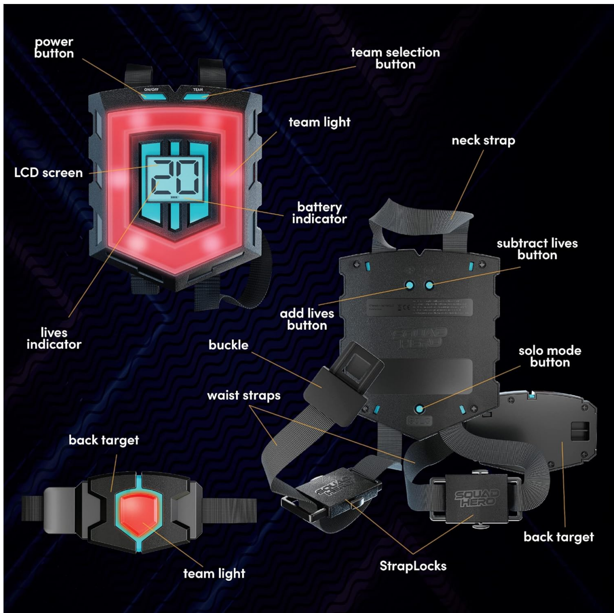
Image: Close-up of the laser tag vest, detailing its components and functions.
