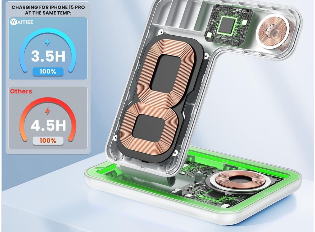
Figure 2: Internal components of the charging station, highlighting charging coils and control chips for efficient power delivery.
