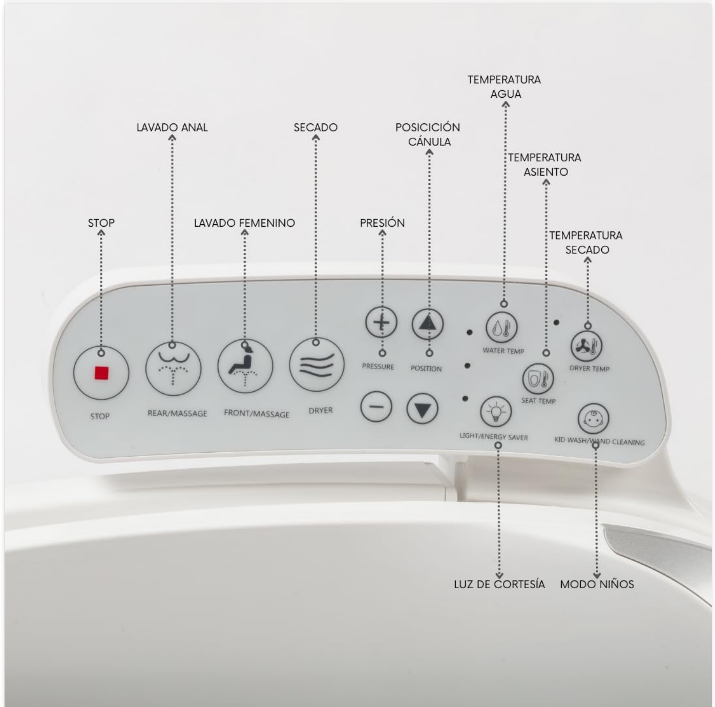
Figure 5.1: Detailed view of the Nashi Compact Pro control panel, showing buttons for Stop, Rear/Massage wash, Front/Massage wash, Dryer, Pressure adjustment, Nozzle Position, Water Temperature, Seat Temperature, Dryer Temperature, Courtesy Light/Energy Saver, and Kids Mode.
