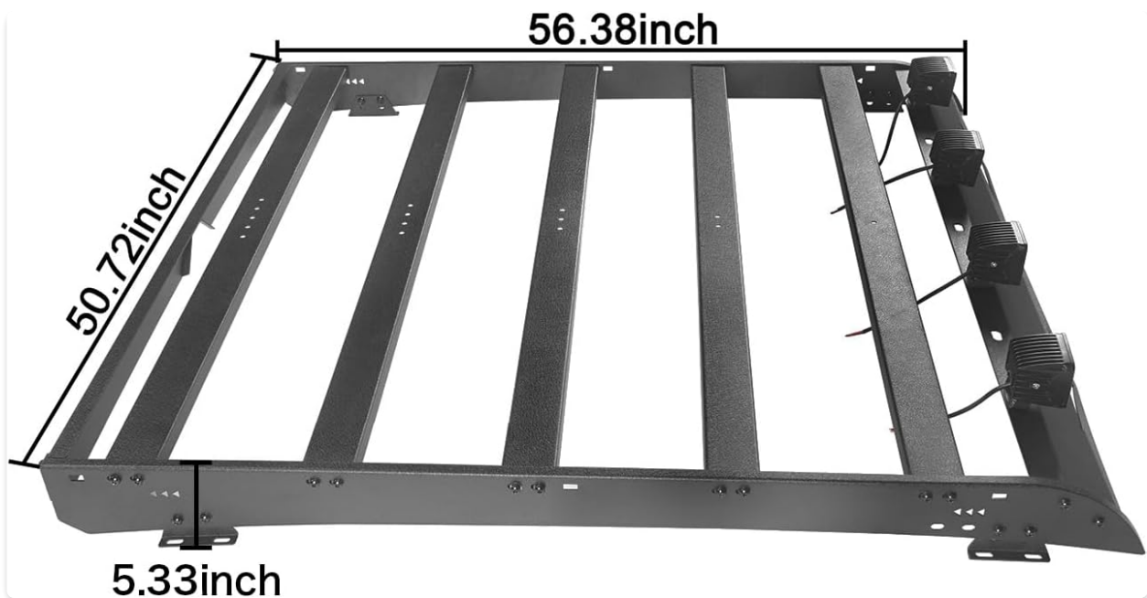
Image 9.1: Dimensional diagram of the roof rack.
