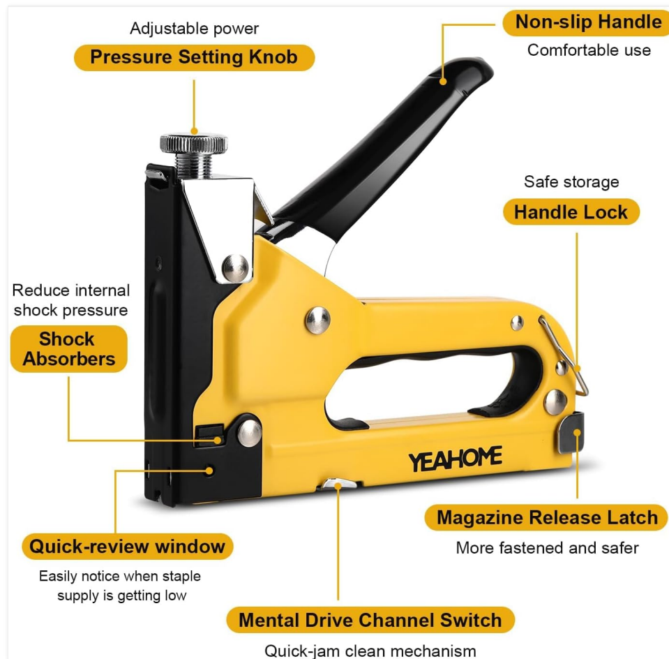
Image 2: Labeled diagram of the staple gun's components.
