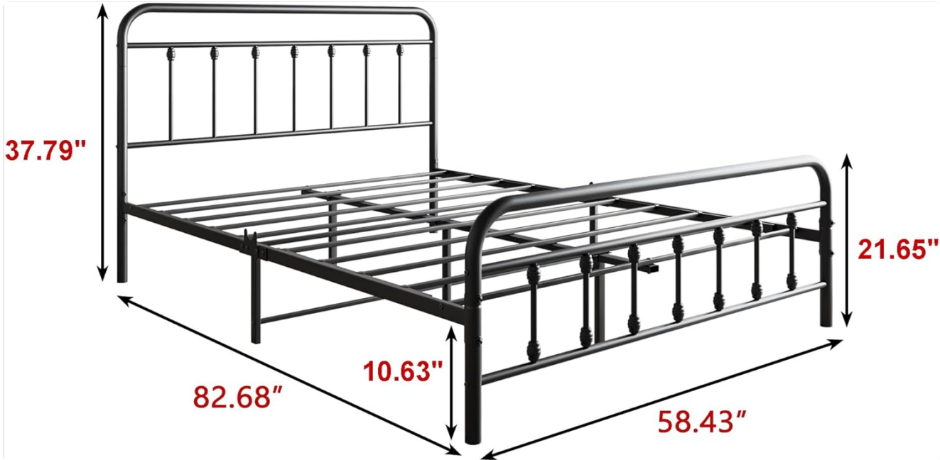
Image: Diagram showing the dimensions of the Elegant Home Products Vintage Queen Size Metal Bed Frame.
