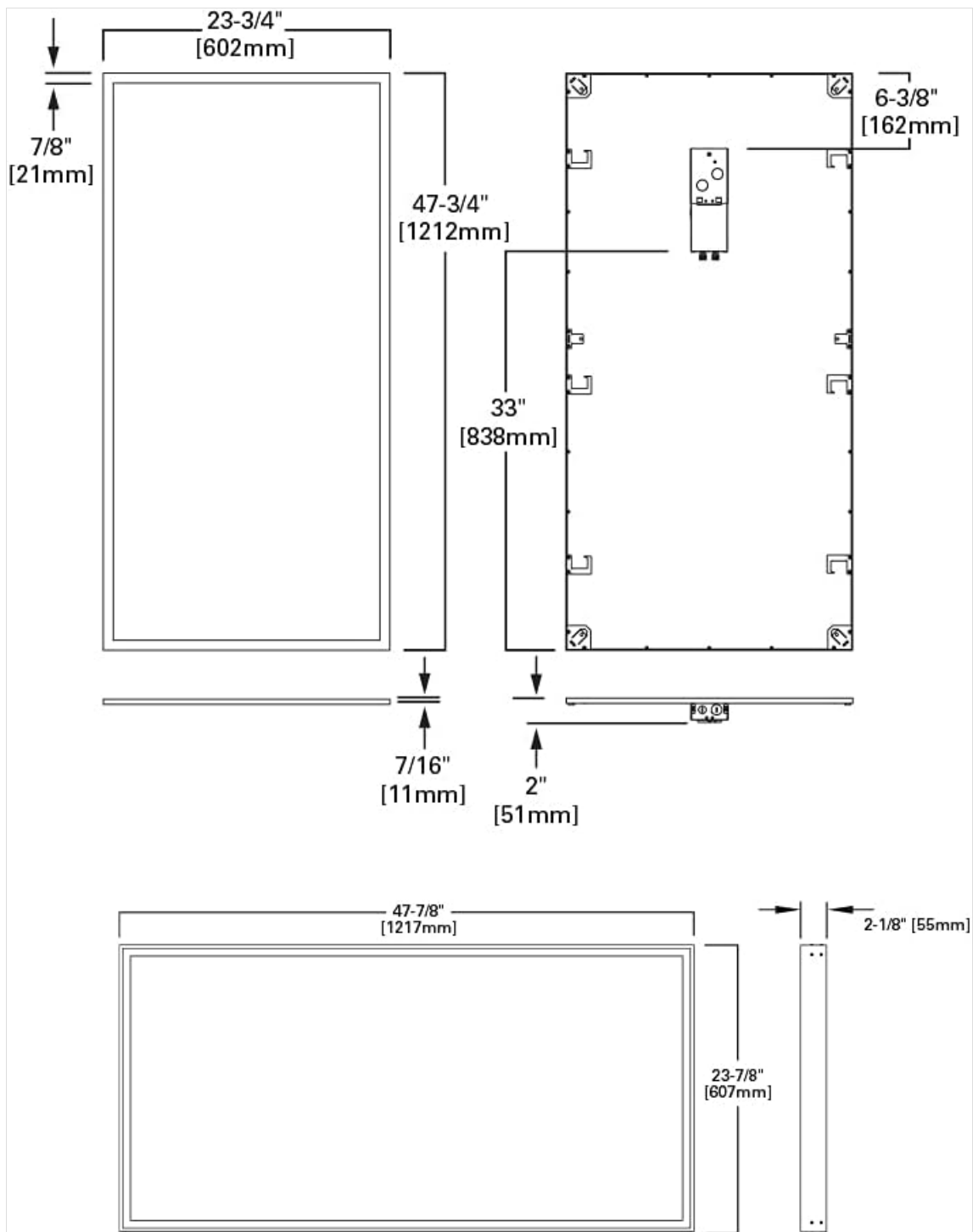
Image: Dimensions of the Metalux 2X4 LED Recessed Panel. This diagram provides critical measurements for proper installation.
