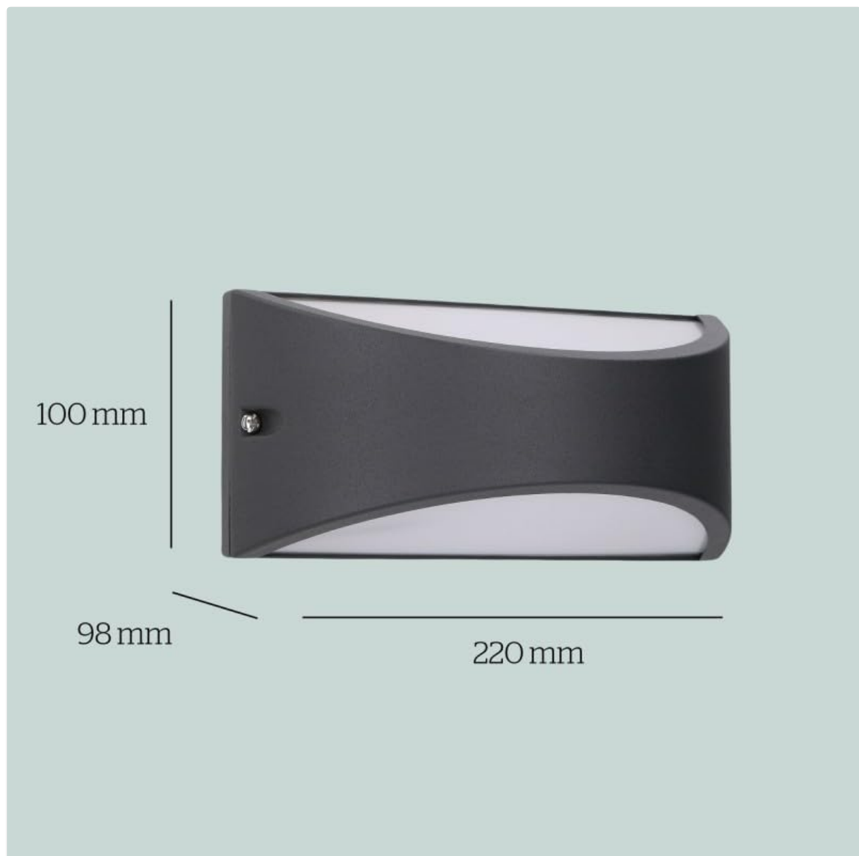
A diagram illustrating the approximate dimensions of the FORLIGHT Kapa LED outdoor wall light: 220 mm length, 100 mm height, and 98 mm depth.
