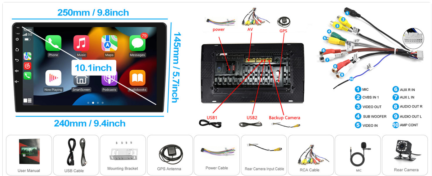
Image: Detailed diagram illustrating the physical dimensions of the car stereo unit and the layout of its rear connection ports for wiring.
