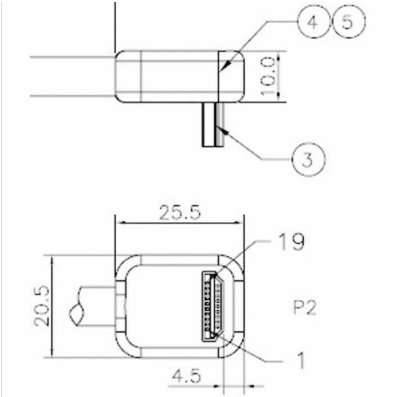
Figure 3: Technical drawing illustrating the dimensions of the HDMI connector, including measurements for width, height, and pin configuration. This diagram provides precise details for compatibility and design.
