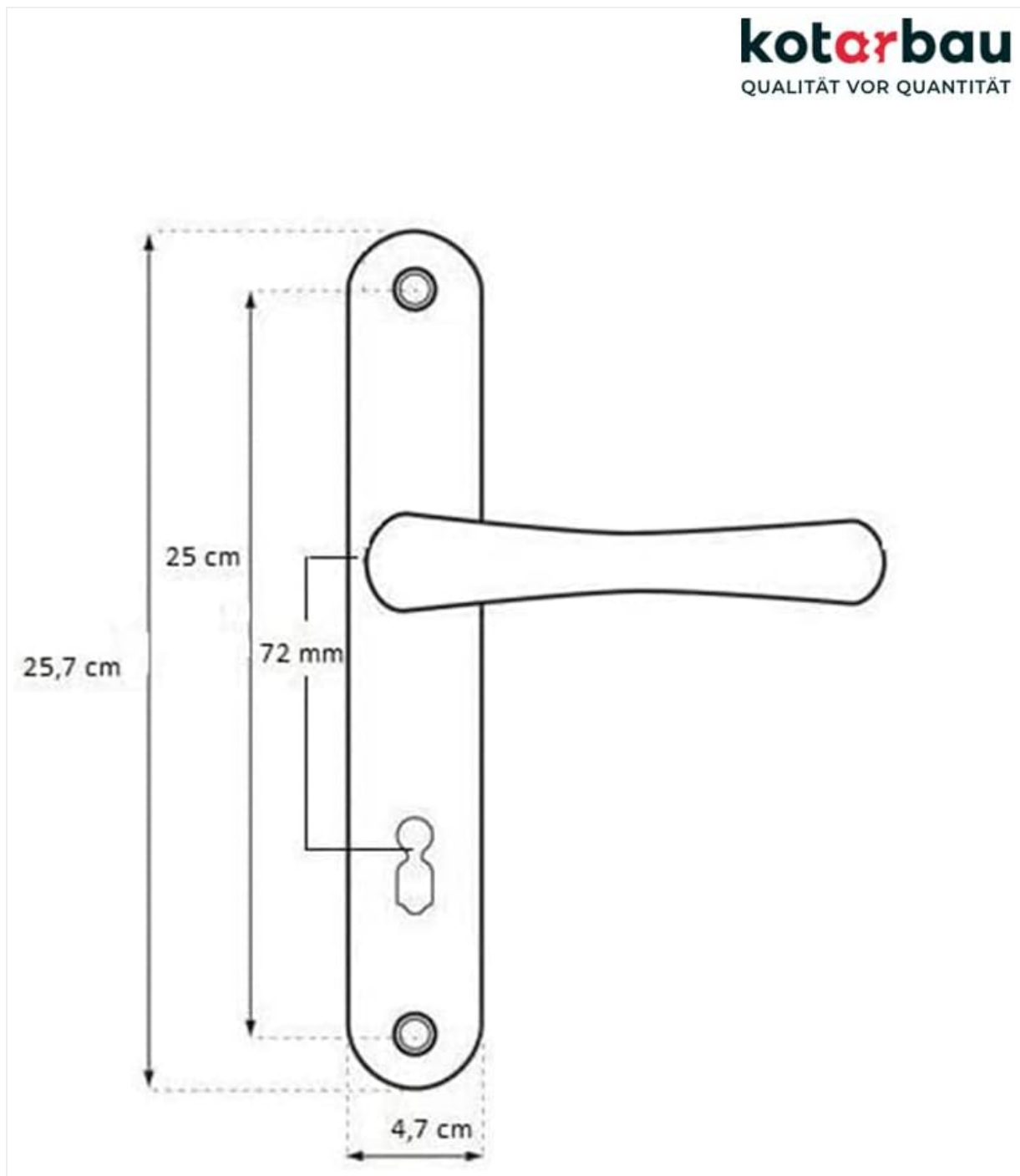
Figure 3: Diagram illustrating the 72mm center-to-center spacing and common lock types (BB, PZ, WC).
