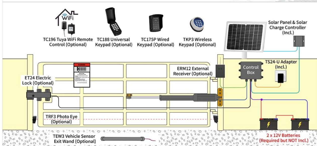
Figure 4: Diagrams illustrating various power supply configurations for the TOPENS A5S.
