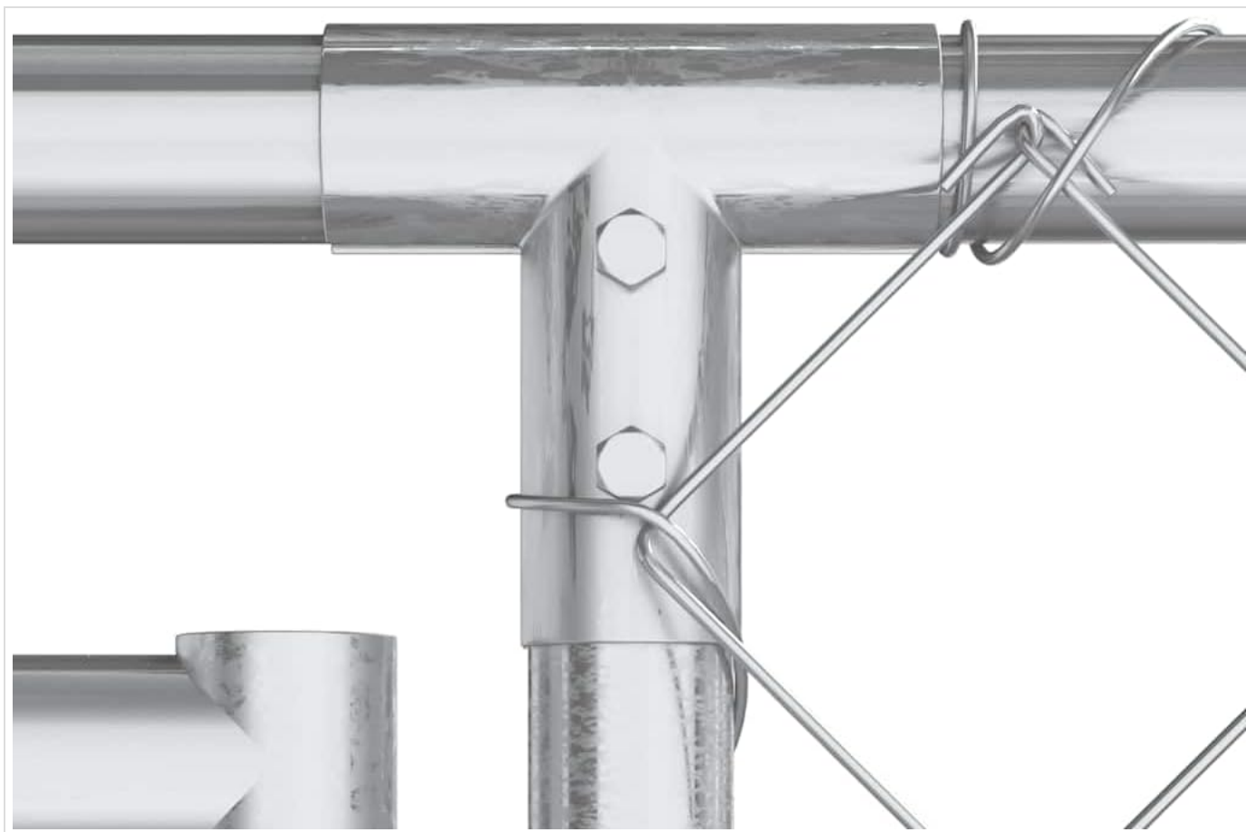
Figure 1: Detail of a T-connector used for frame assembly. Ensure bolts are loosely fitted initially.
