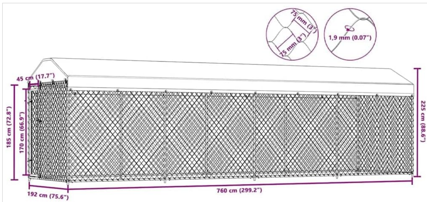
Figure 4: Detailed dimensions of the dog kennel, including height, width, and length.
