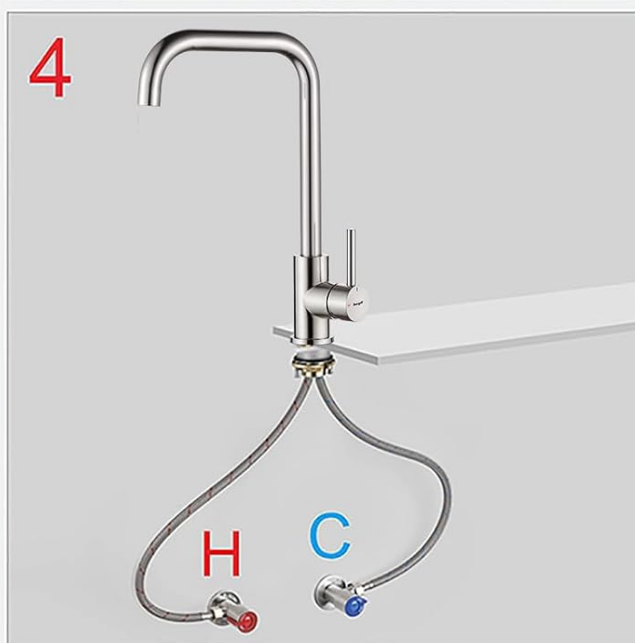
Image: Four-step visual guide demonstrating the installation process of the kitchen faucet, from inserting the faucet to connecting the water lines.
