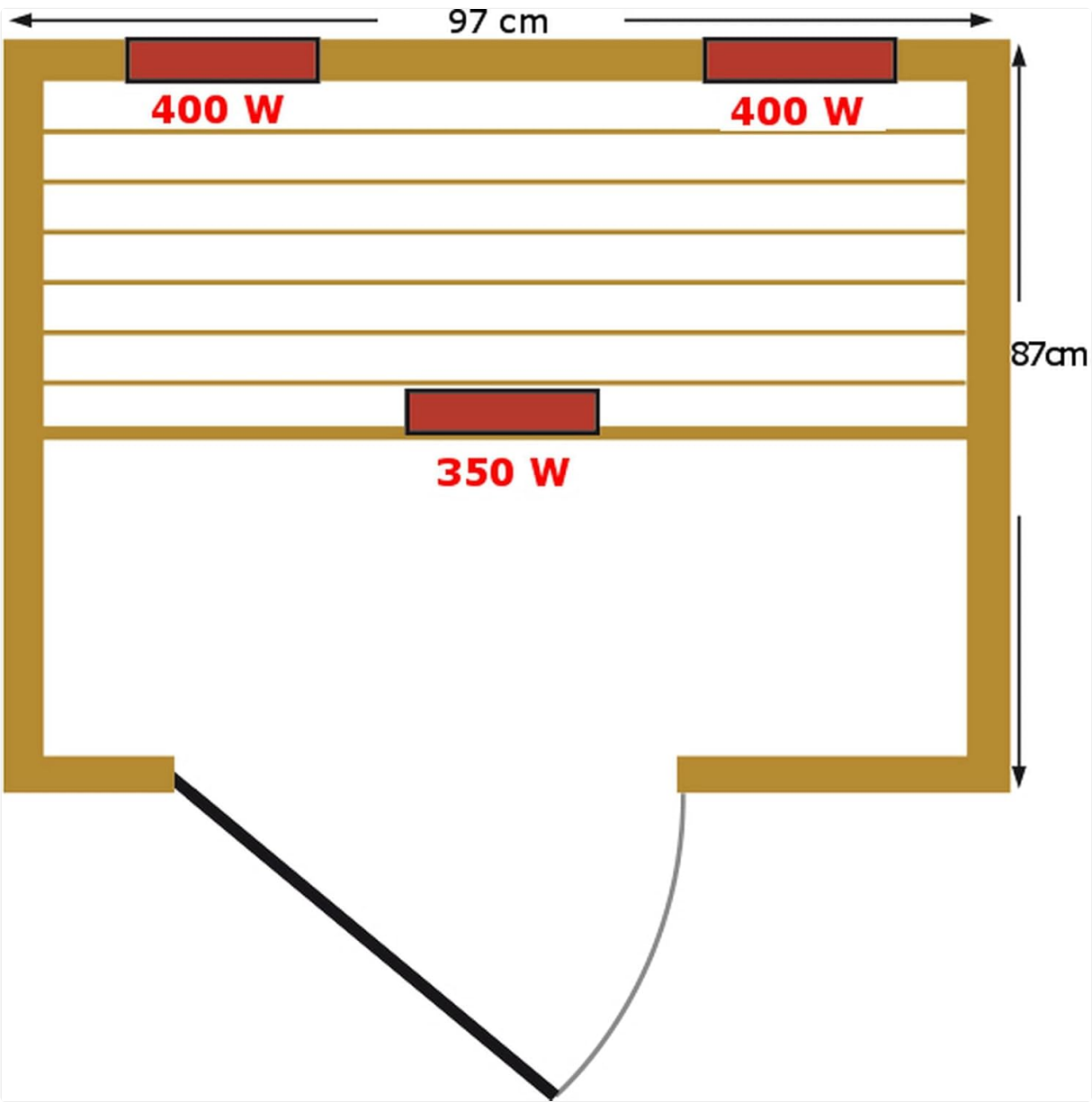
Figure 6: Top-down schematic showing the placement of the three ceramic heaters: two 400W heaters on the back wall and one 350W heater below the bench, totaling 1150W (1.15 kW).
