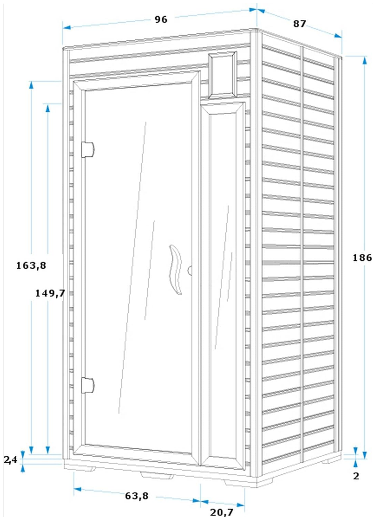
Figure 3: Technical drawing illustrating the external dimensions of the sauna: 97 cm (width) x 87 cm (depth) x 186 cm (height).
