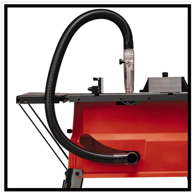
Figure 3.5: View of the dust extraction system, including the hose connecting to the saw blade area and the main collection port.
