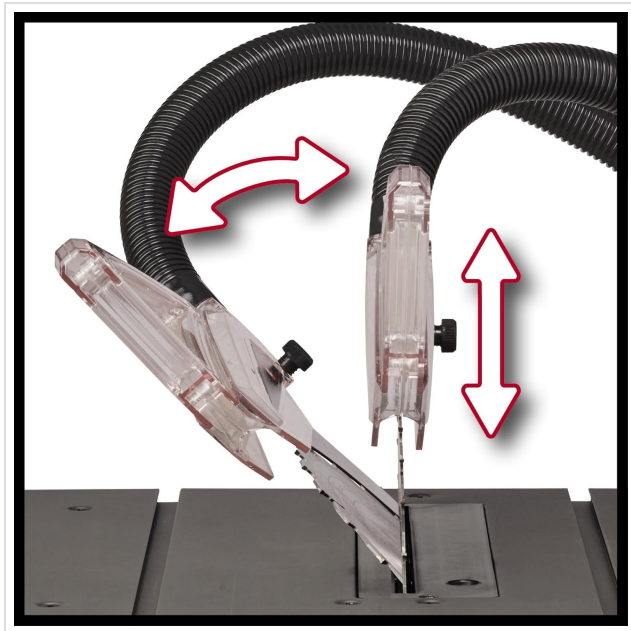
Figure 3.4: Detail of the saw blade guard and the flexible hose for dust extraction, showing height and angle adjustment indicators.
