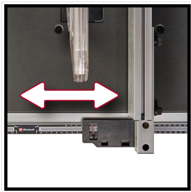
Figure 3.6: Close-up of the parallel stop with its integrated measurement scale for accurate longitudinal cuts.
