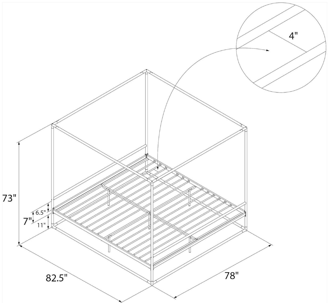
Image: Detailed assembly diagram showing the structure and dimensions of the bed frame.
