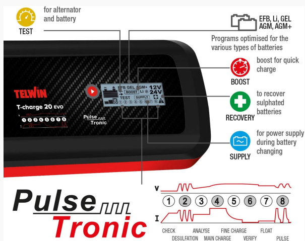
Figure 3.2: Close-up view of the charger's LCD display, indicating battery type, voltage (12V/24V), and charging status with numbered steps (1-8).
