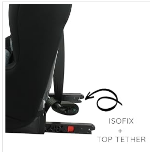
Figure 4.1: Detail of the Isofix connector mechanism.
