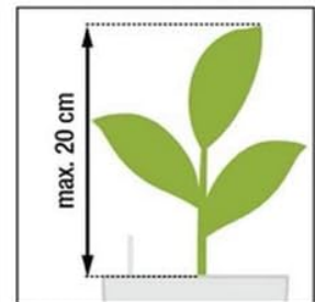
Image: A diagram illustrating the dimensions of the OJO planter (21 cm diameter, 15.8 cm height), the water reservoir capacity (0.25 liters), and the recommended plant pot size (10-12 cm diameter, max 20 cm height).
