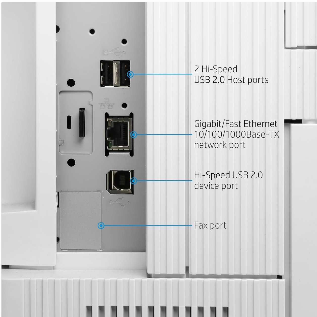
Figure 4.3: Rear view of the printer showing available connectivity ports.
