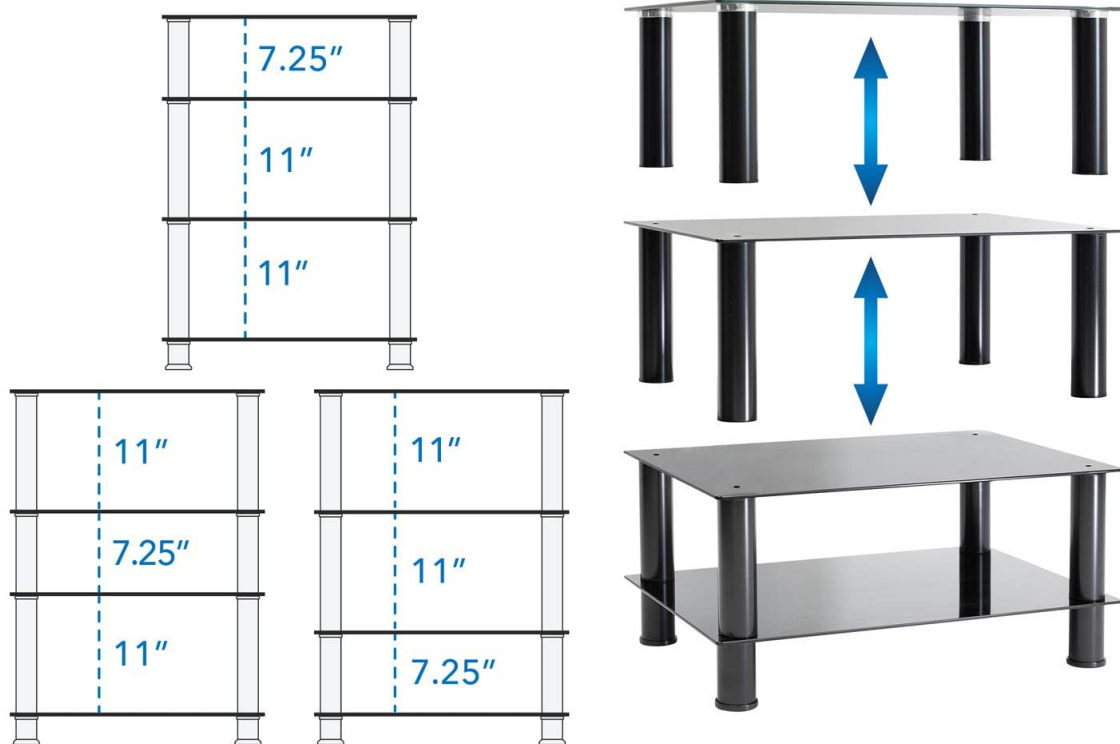
Figure 2: Adjustable Shelving. The modular design allows for customization of shelf heights to accommodate various AV components.
