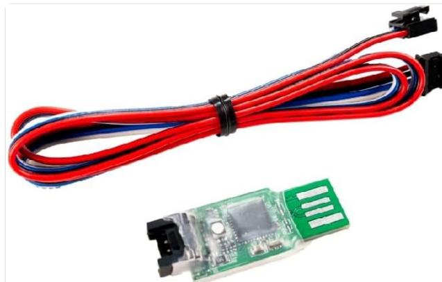
Figure 4: The data module and its associated wiring harness, which simplifies the installation by reducing the number of required wiring connections.
