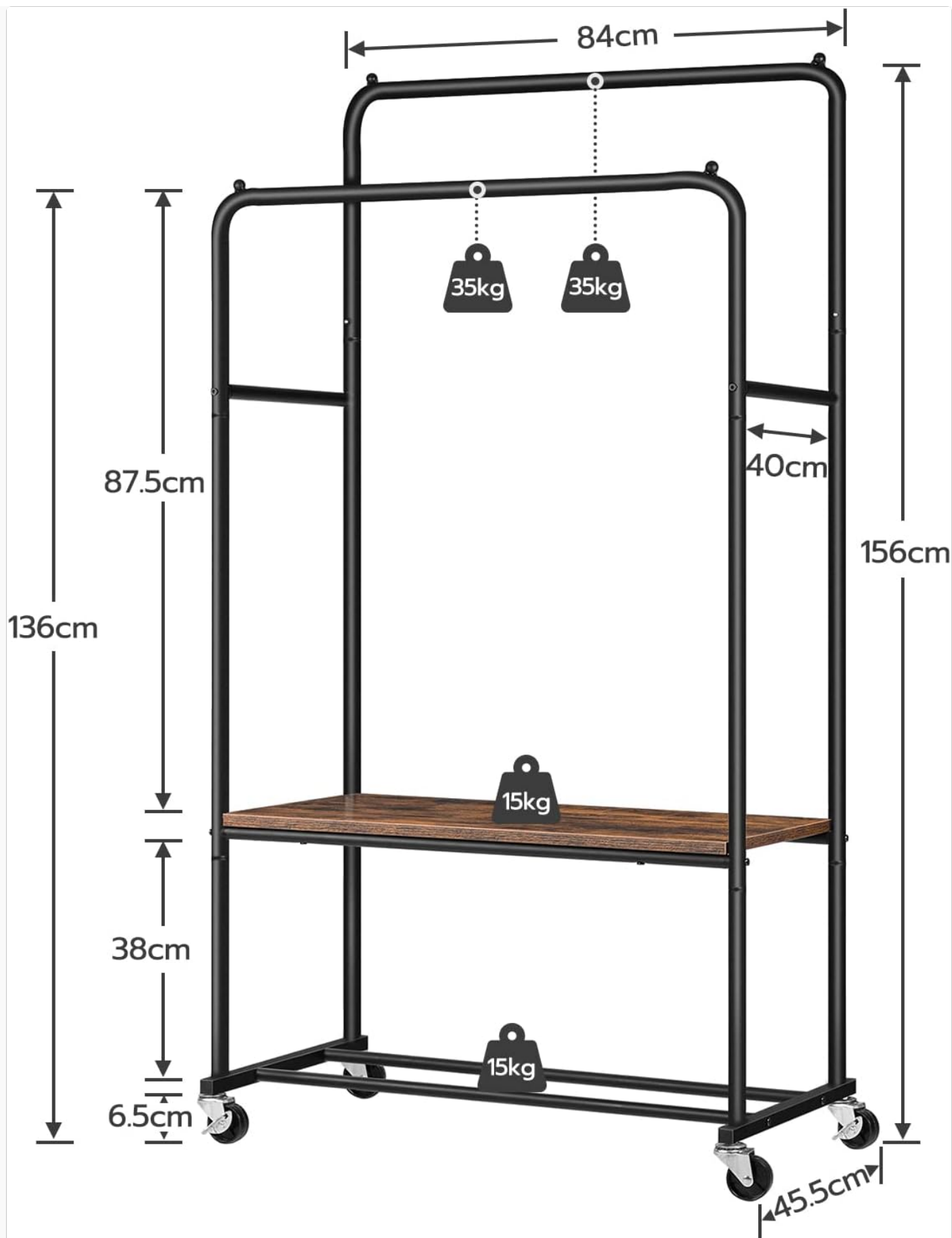
Image: Detailed diagram illustrating the dimensions (84cm width, 156cm height, 45.5cm depth) and individual weight capacities for the hanging rails (35kg each) and shelves (15kg each) of the clothes rack.
