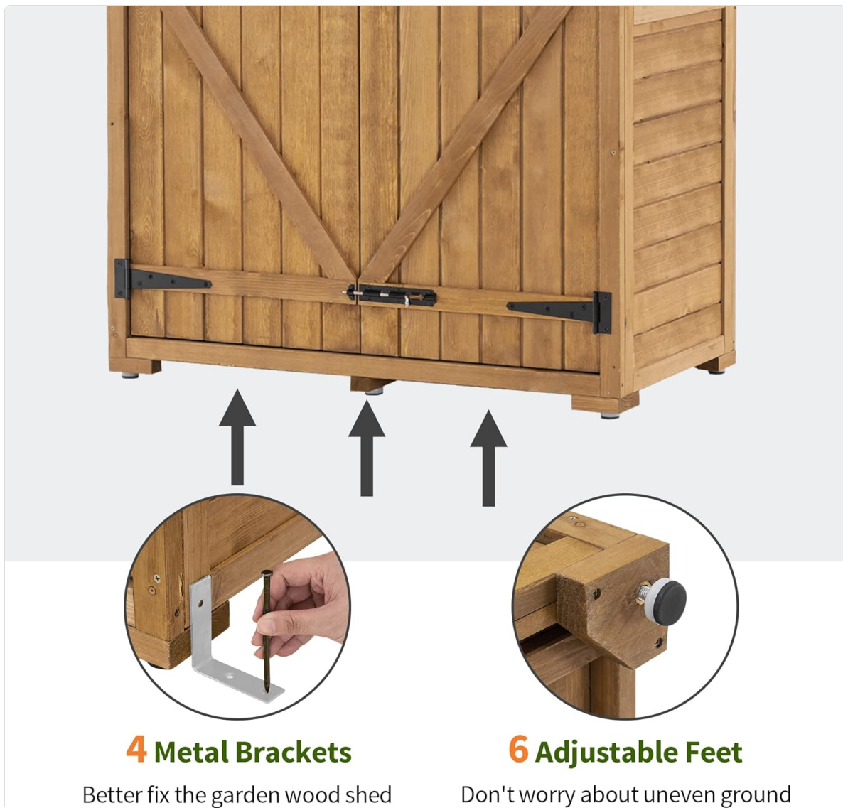
Image 5.1: Illustration of the 4 metal brackets for securing the shed and the 6 adjustable feet for leveling on uneven ground.
