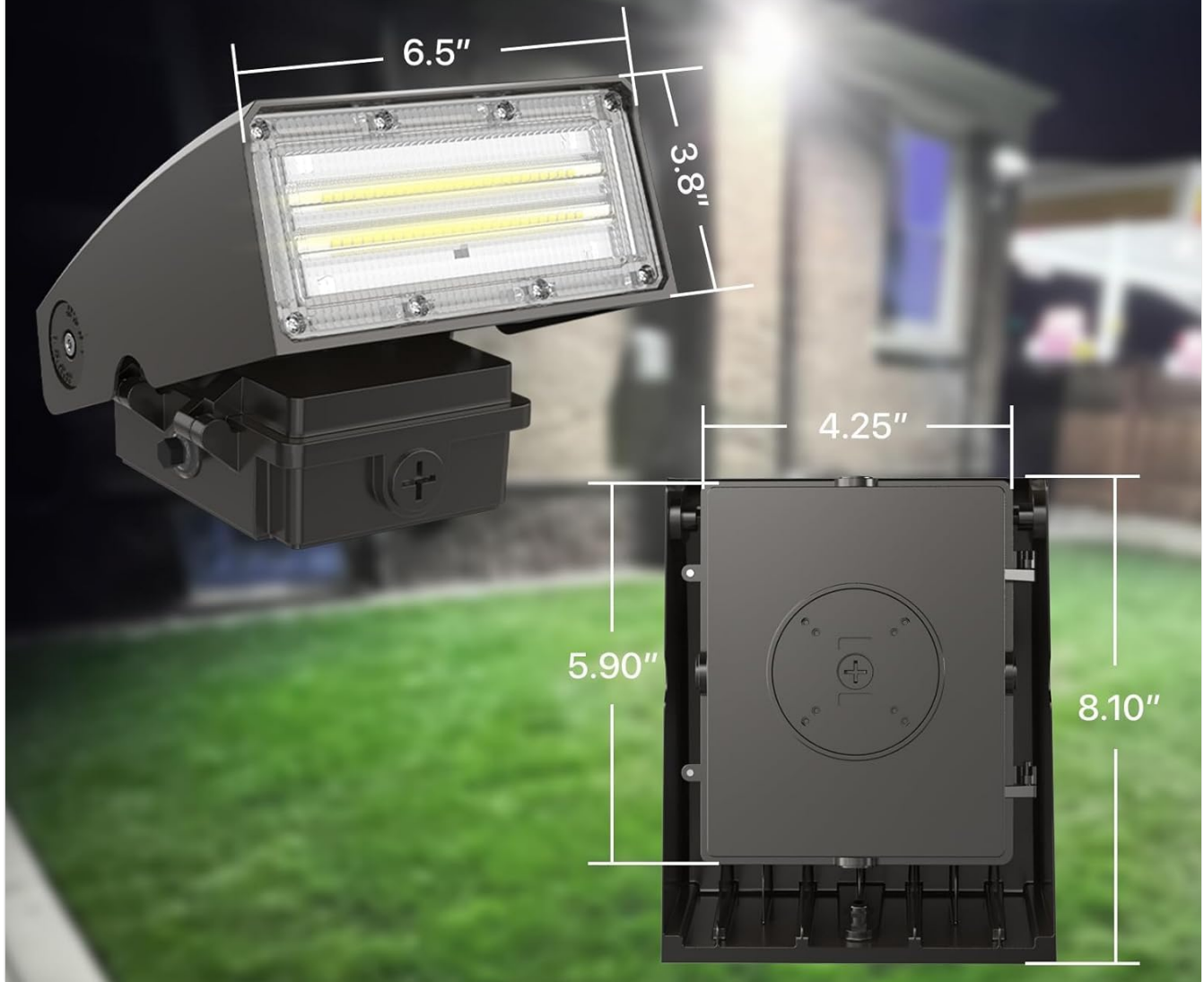
Figure 3.1: Product Dimensions.
